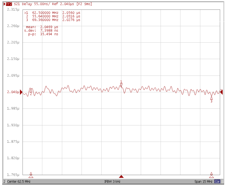
Group Delay Variation Fo±6.86 MHz
