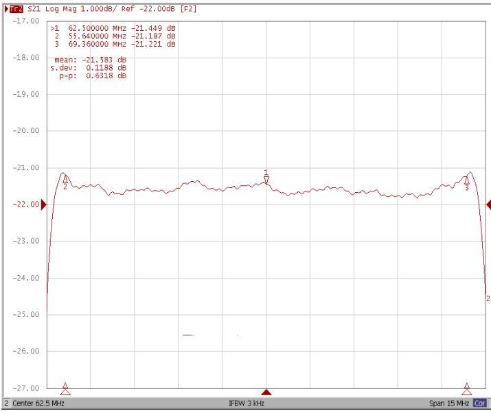
Ripple Variation Fo±6.86 MHz
